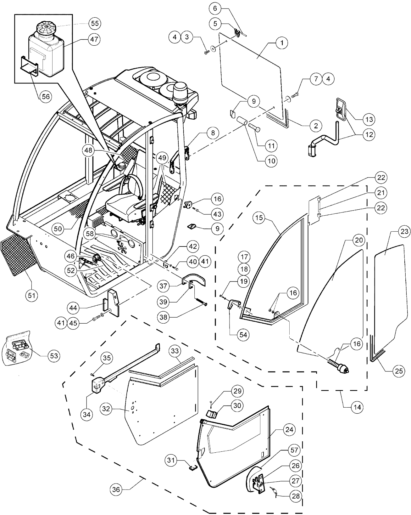
402.1 605671 Cabin, View 2
